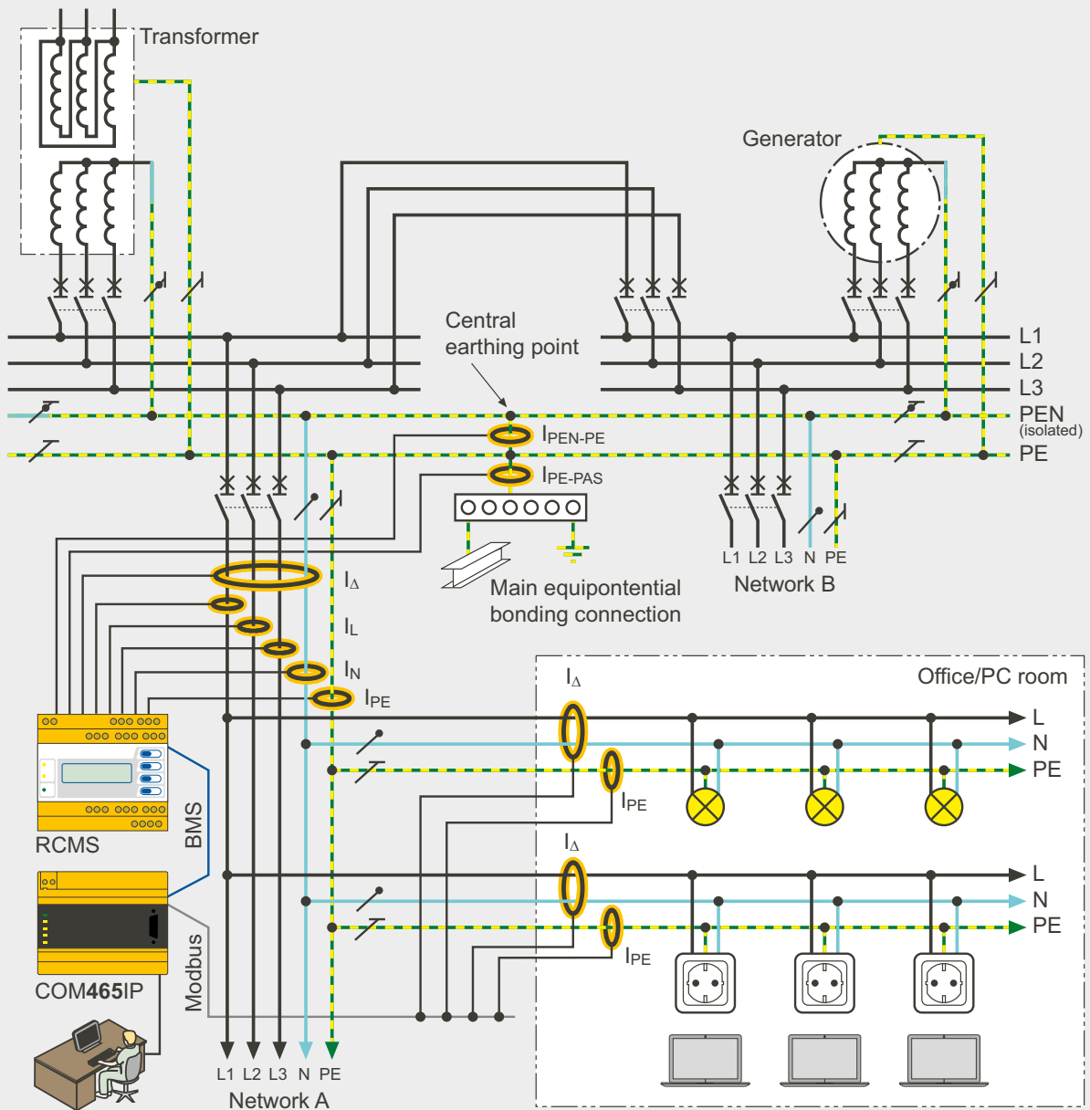
Power supply in an office building
